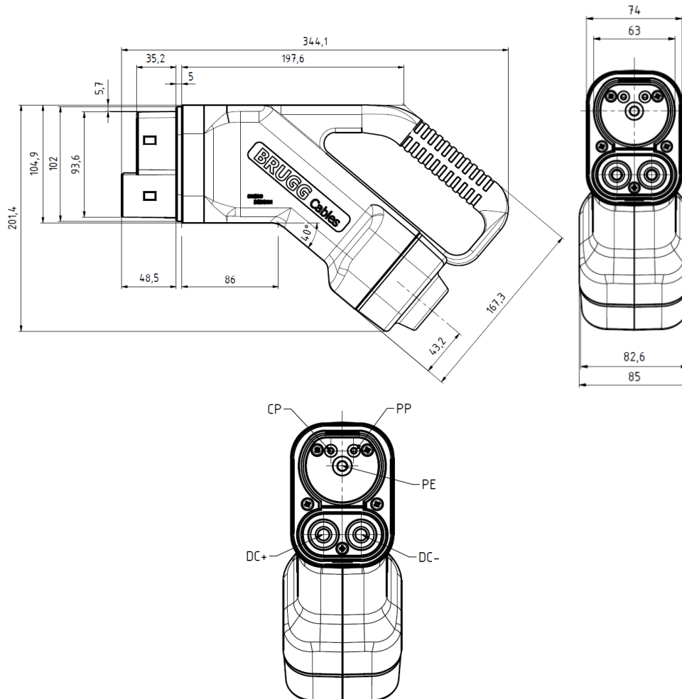
Pin distribution, CCS-2 Connector
